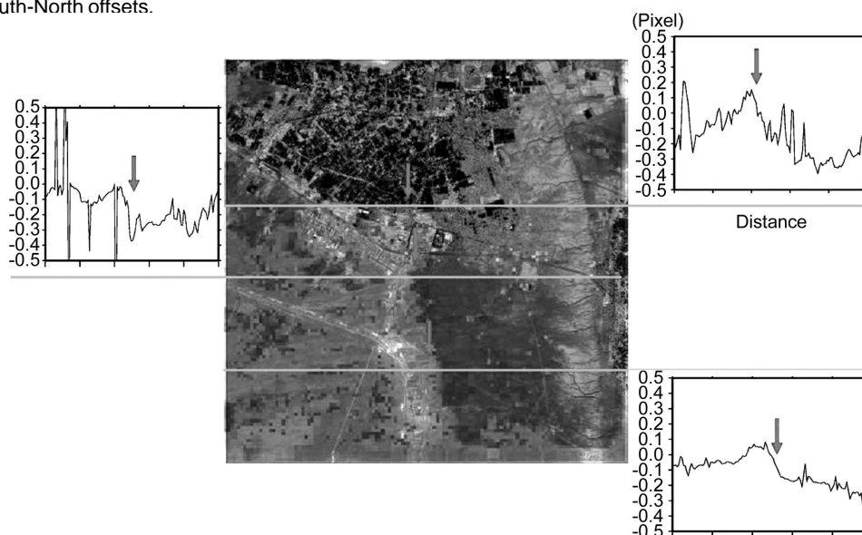
Figure 7. 3 profiles of the S-N Spot offsets across the rupture south of Bam. The relative change across the fault is estimated to one third of a pixel size (~80cm).
