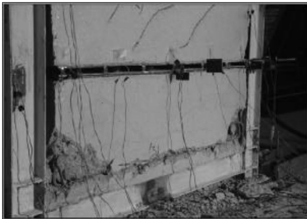
(a) Infill Cracking and Crushing
