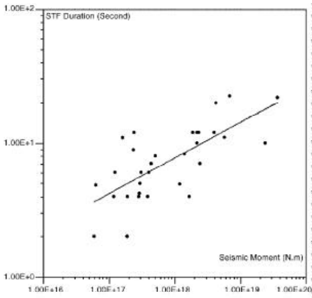
Figure 7. Source duration ( \tau_i ) versus seismic moment ( M_0 ).
