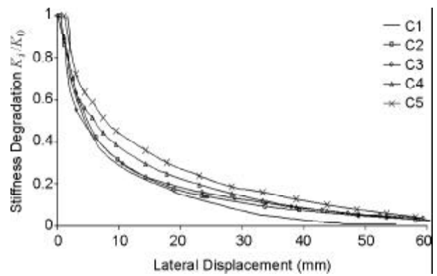
Figure 11. Stiffness degradation of columns.
