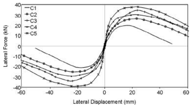
Figure 8. Envelope curves.
