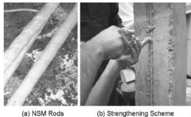
Figure 5. Strengthening techniques.
