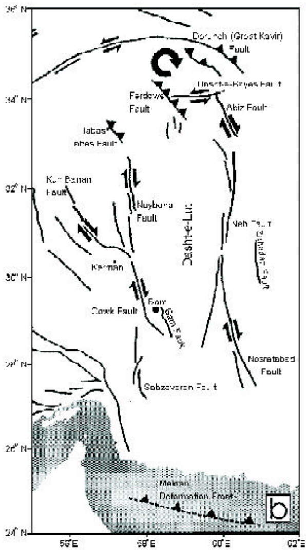
Figure 1. Major N-S trending, right lateral strike slip fault systems in eastern Iran [17].
