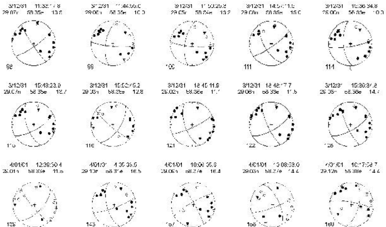
Appendix I: Lower-hemisphere equal-area fault plane solutions for selected aftershocks. Compressional first motions are shown as solid circles, dilatation first motion as open circles. P-axes are shown as solid triangles and T-axes as open triangles.
